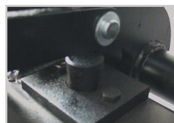
1 ½" diameter heat treated scarifier locking pin
